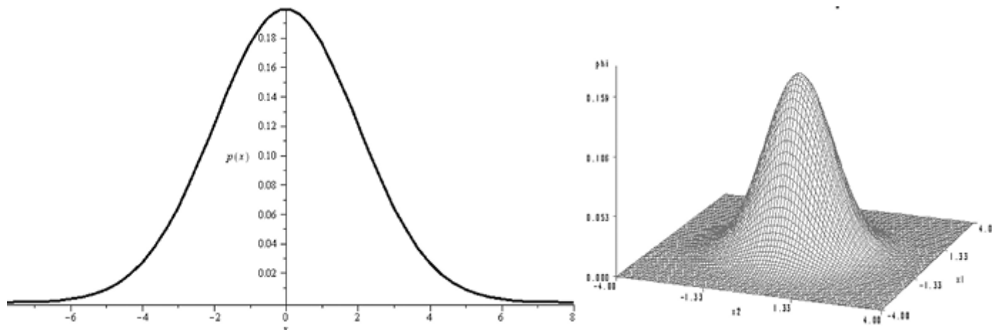
Figure 7-7 : A univariate bell curve (left) and a bivariate bell curve (right)
