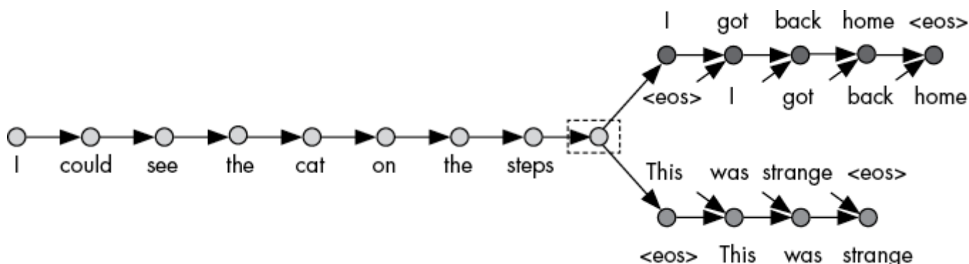
Figure 10-2 : We use the skip-thoughts model to predict which sentences appear near each other.
